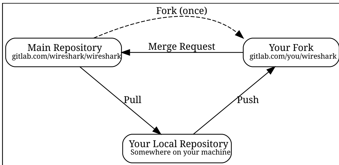
Figure 1. GitLab Workflow
